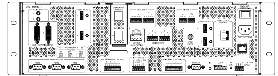
DVX-2155HD-T REAR VIEW
