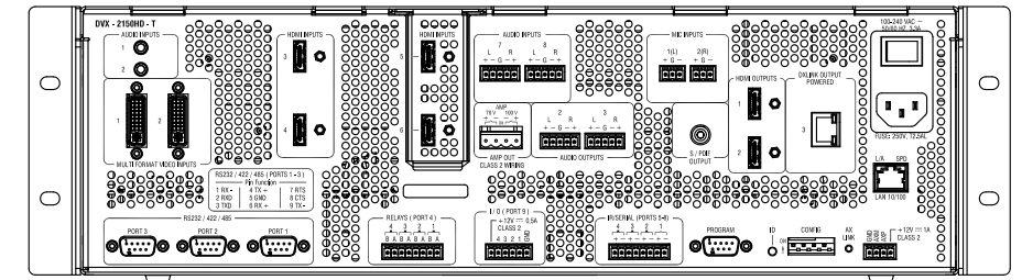
DVX-2150HD-T REAR VIEW
