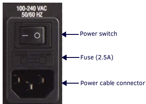
FIG. 58 Power Connector/Switch/Fuse
