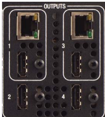
FIG. 40 Video Outputs
