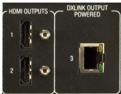
FIG. 41 Video Outputs
