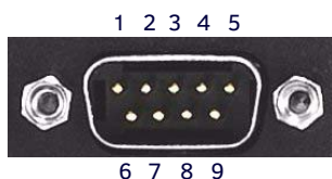
FIG. 45 RS-232/422/485 (DB9 - male) Connector Pinouts
