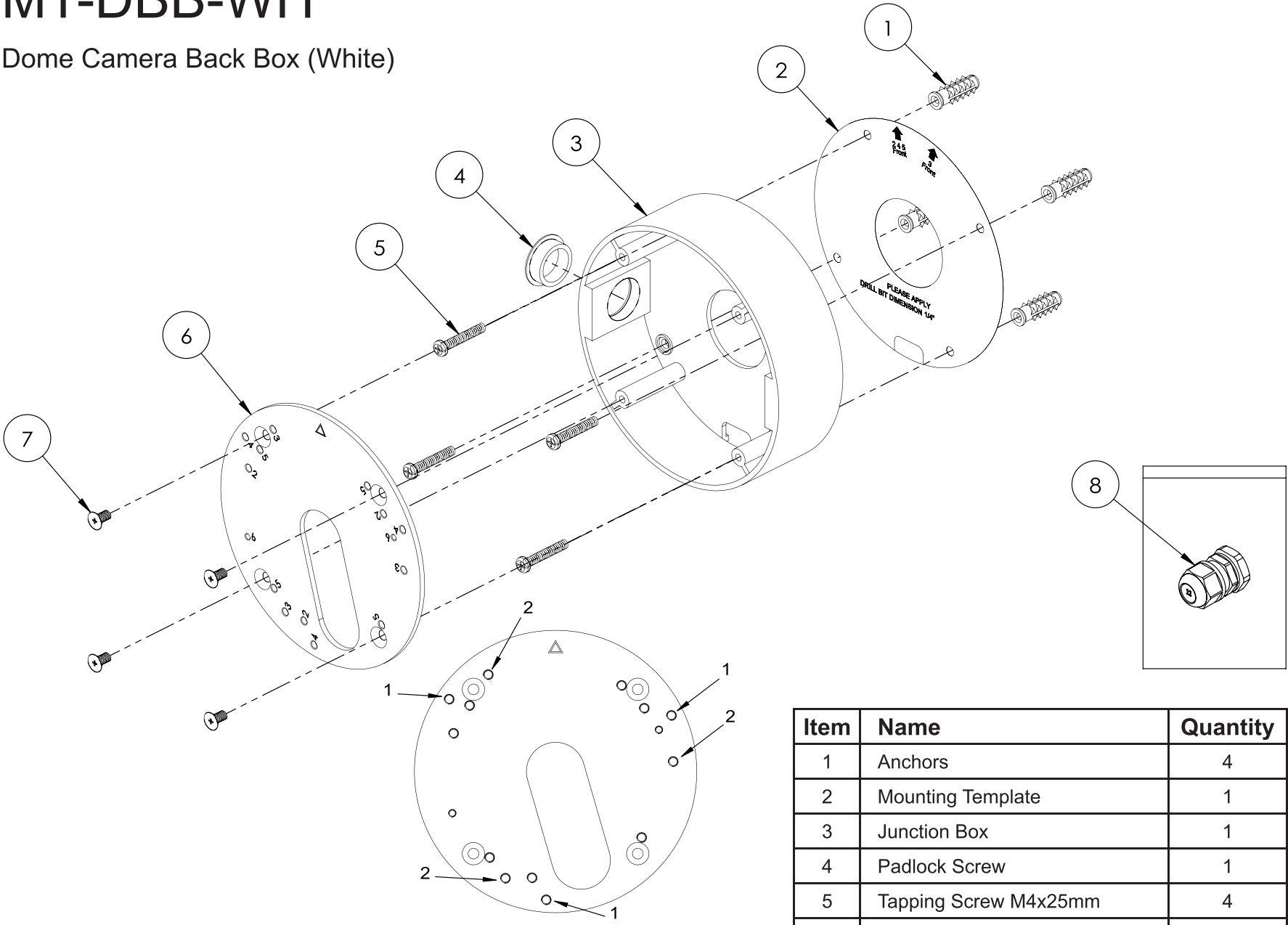
Hole Position Diagram
