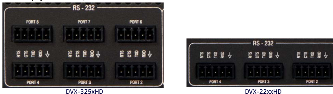
FIG. 46 RS-232 ports
