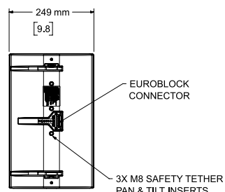
Rear View BRACKET REMOVED FOR CLARITY
