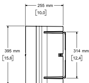
Right View DIMENSIONS APPLY TO BOTH SIDES
