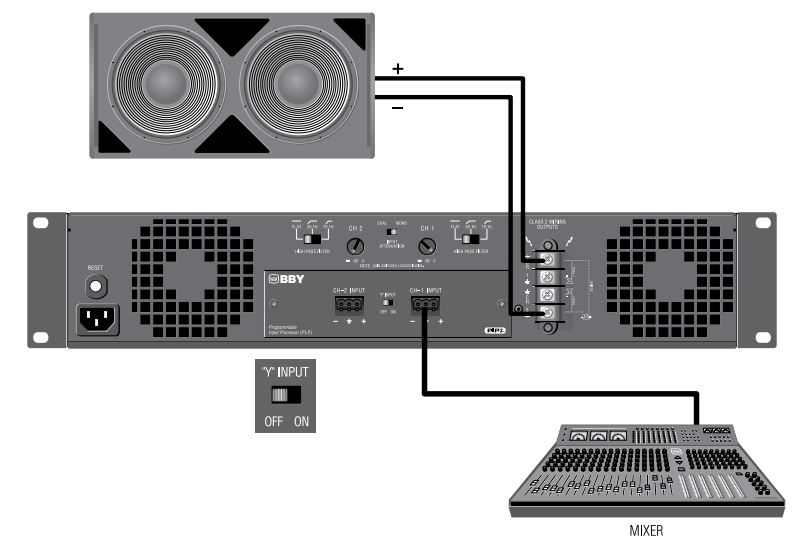
Figure 3.9 System Wiring, Bridge-Mono Mode
