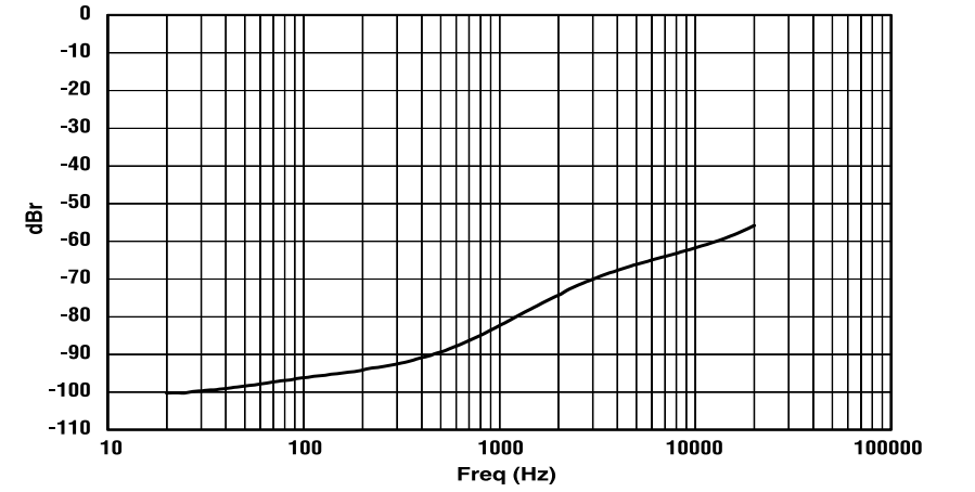
Figure 7.5 CTs 2000/3000 Typical Crosstalk vs. Frequency
