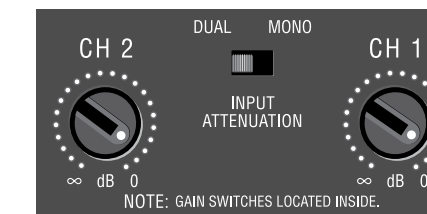
Figure 3.8 Attenuator and Mode-Switch Settings for Dual Mode
