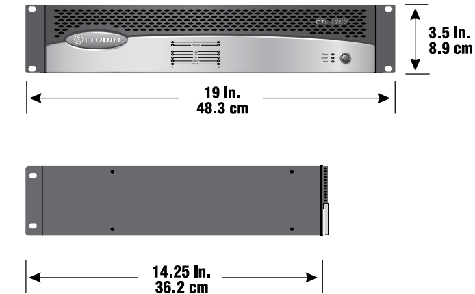
Figure 3.1 CTs 2-Channel Series Dimensions
