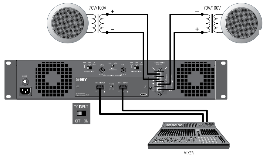
Figure 3.11 System Wiring and Y-Switch Setting for 70V/100V Operation
