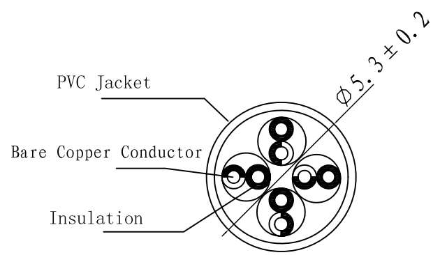
Cable Section: A-A
